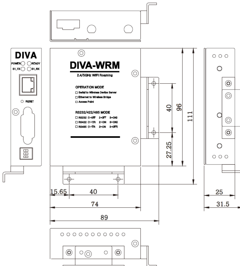
Panel/Wall Bracket
